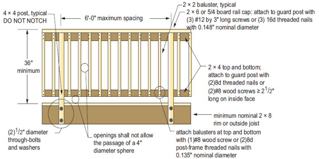
FIGURE 6-23 Example guard detail.
